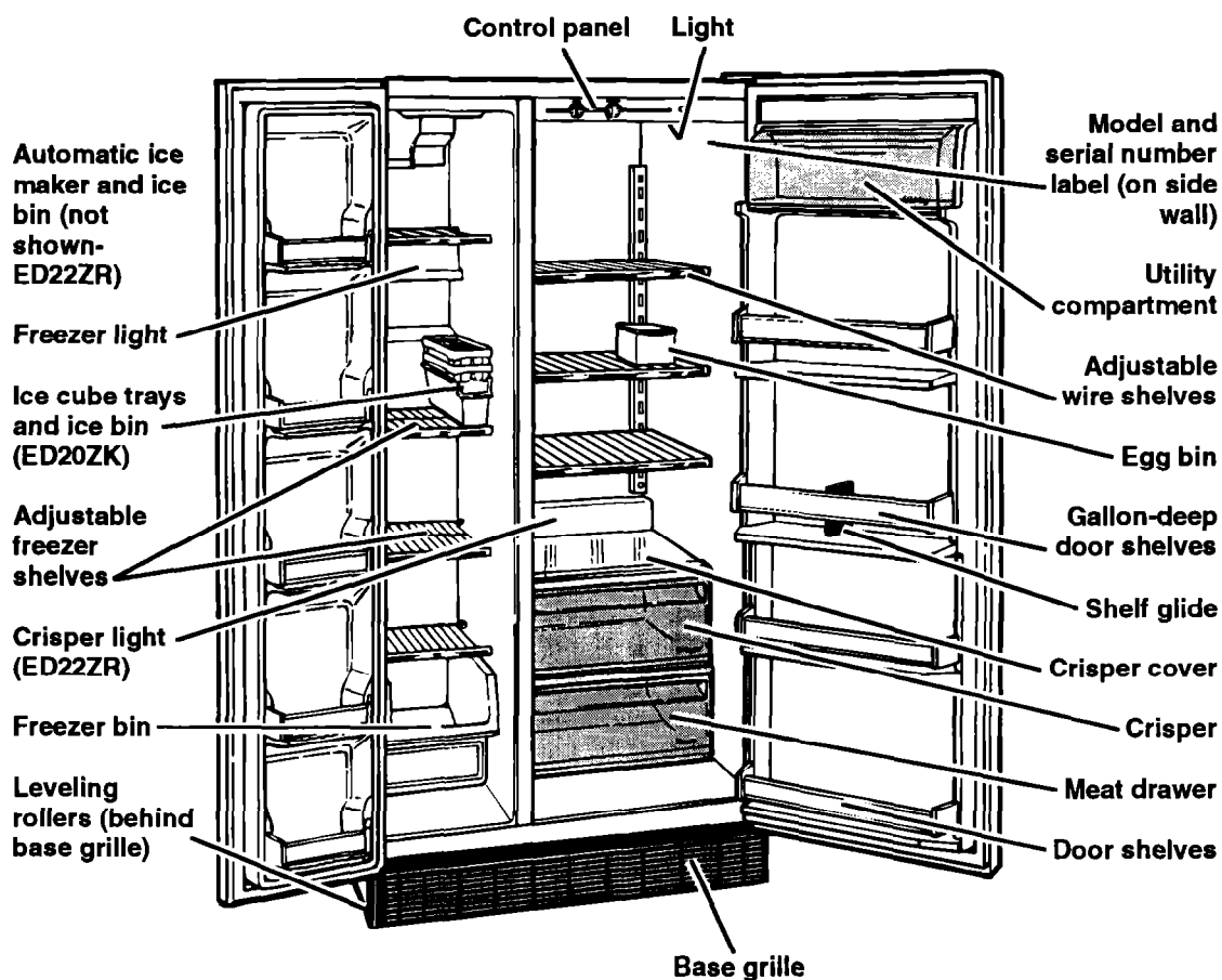
Model ED20ZK shown
