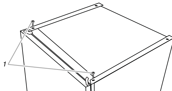
1. Remove screws
