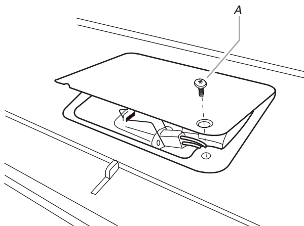
A. Bulb cover mounting screw
